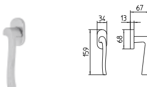
1072/DK MARTELLINA DK drehkipp system
