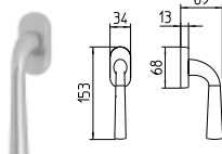
S102/DK MARTELLINA DK drehkipp system
