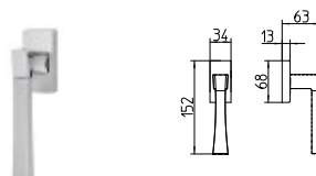
1172/DK MARTELLINA DK drehkipp system
