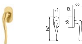
S72/DK MARTELLINA DK drehkipp system
