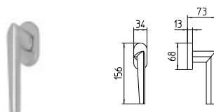
1082/DK MARTELLINA DK drehkipp system
