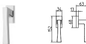
1162/DK MARTELLINA DK drehkip system
