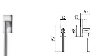
1462/DK MARTELLINA DK drehkipp system
