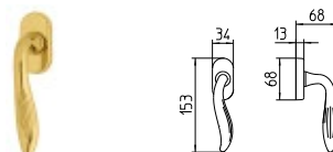
982/DK MARTELLINA DK drehkipp system
