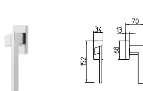
1372/DK MARTELLINA DK drehkipp system
