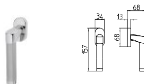
362/DK MARTELLINA DK drehkipp system
