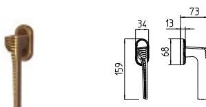
1362/DK MARTELLINA DK drehkipp system
