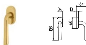
S62/DK MARTELLINA DK drehkipp system
